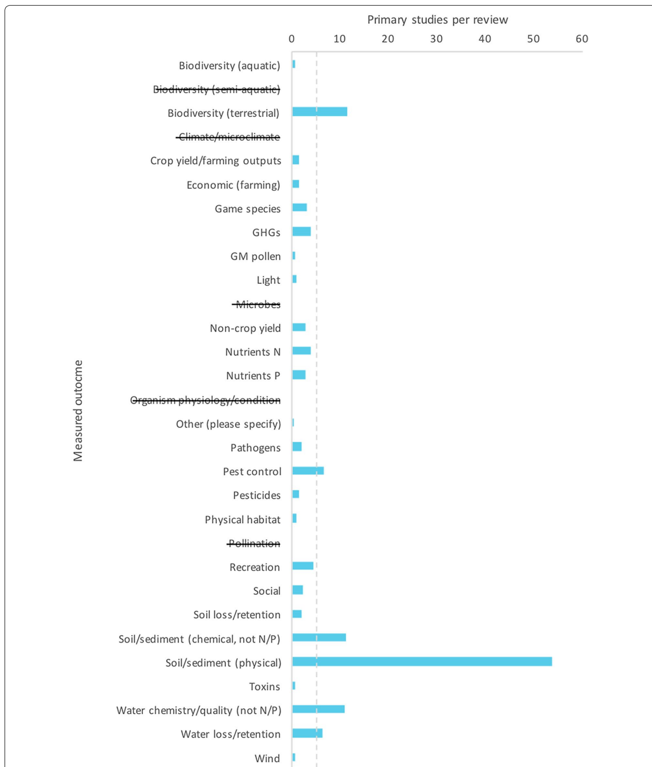
Fig. 28 The number of primary studies per review article reporting each outcome, displaying the mean study:review ratio of 5.4 as a dashed grey line. Outcomes that are struck through represent those for which no reviews were identified
